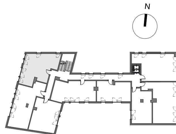
PIĘTRO +1
