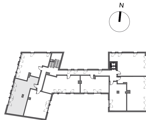
PIĘTRO +1
